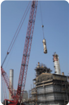
Waste Heat Recovery Boiler Replacement -PPL Goa Unit
